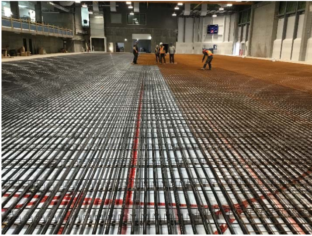
Brine Lines – 15.5 kilometers of brine lines are covered with rebar mesh.
