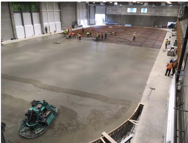
Slab Pourt – Crew works on pouring the 5" thick concrete arena slab.
