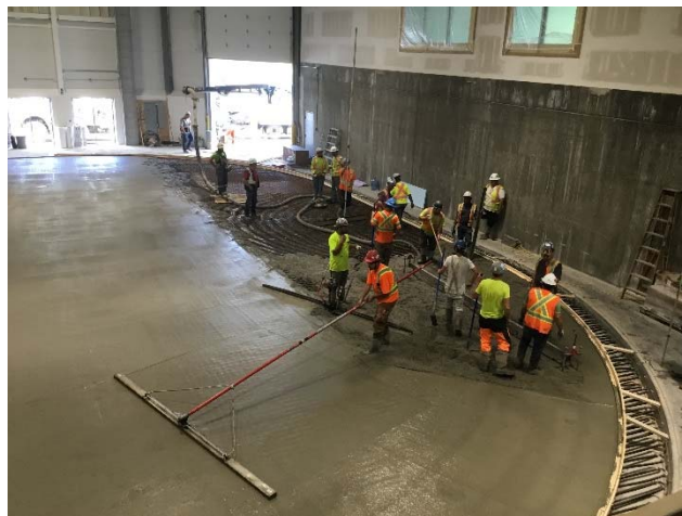
Almost There – Crew works on last section of slab pour.
