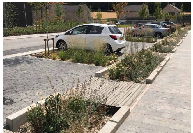
Figure 30: Design parking areas to maximize rainwater infiltration.
